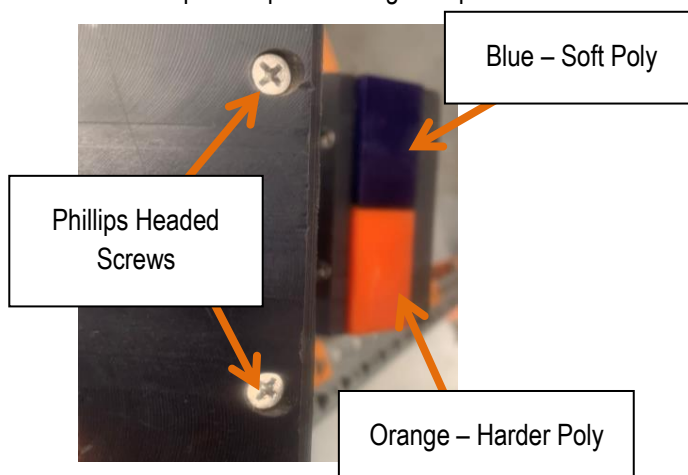
Figure 7 - Poly Pad Replacements
