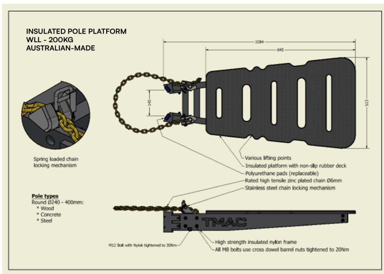
Figure 1 – 1050mm Insulated Pole Platform Details
