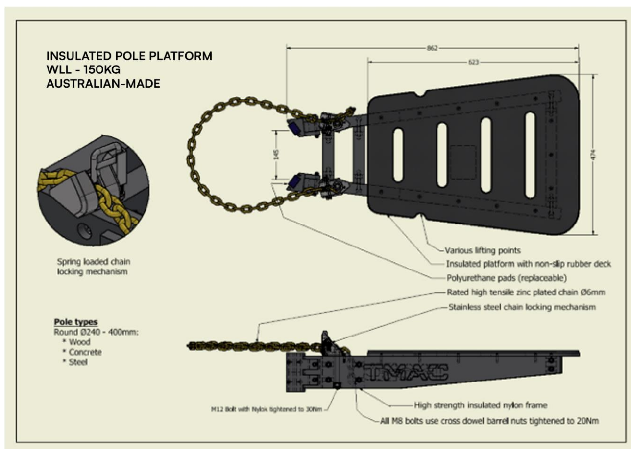
Figure 2 - 850 Insulated Pole Platform Details
