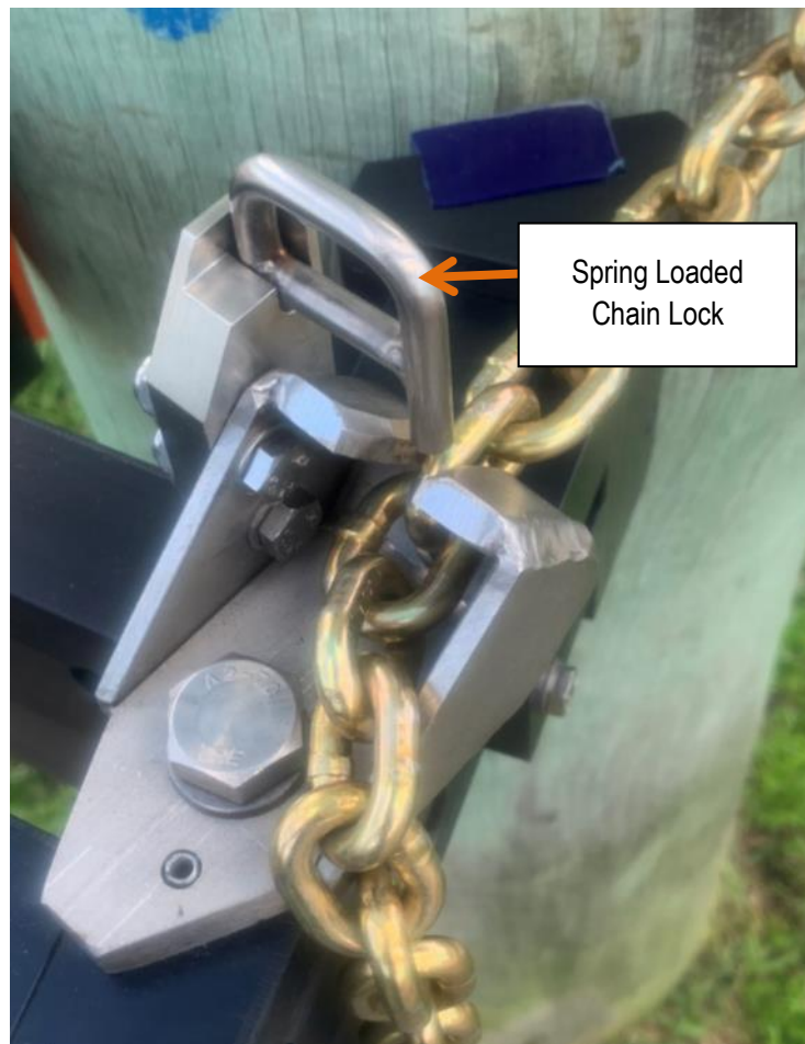
Figure 6 - Spring Loaded Chain Locking Mechanism
